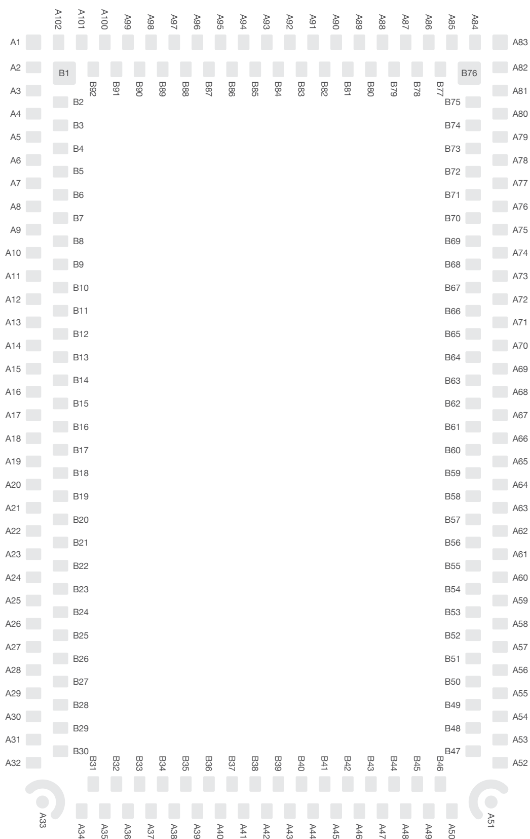
FIGURE 3-1. PIN ASSIGNMENTS
