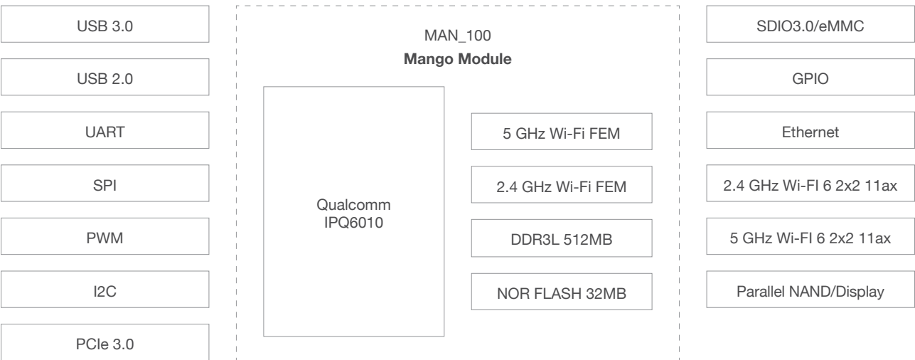
FIGURE 2-1. BLOCK DIAGRAM
